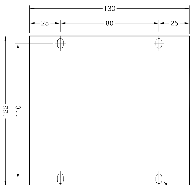
MOUNTING
